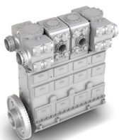
LABY COMPRESSORS Contactless and Oil-Free
